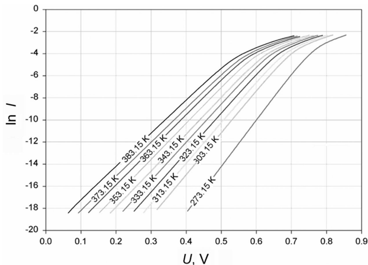
Fig. 2. I-U characteristics at different temperatures.
