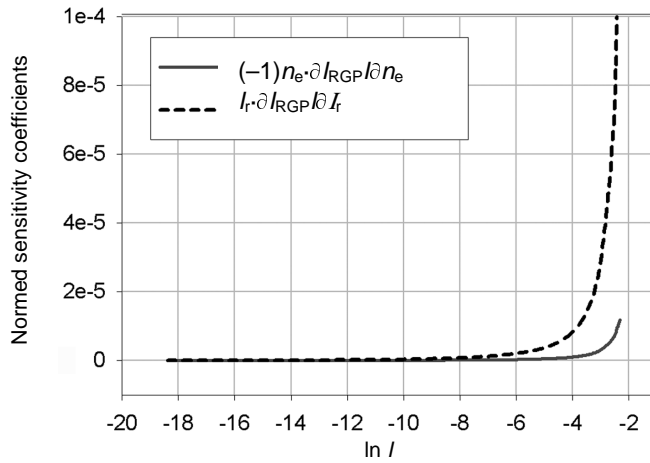
Fig. 7. Sensitivity analysis of the RGP model (Part 2).
