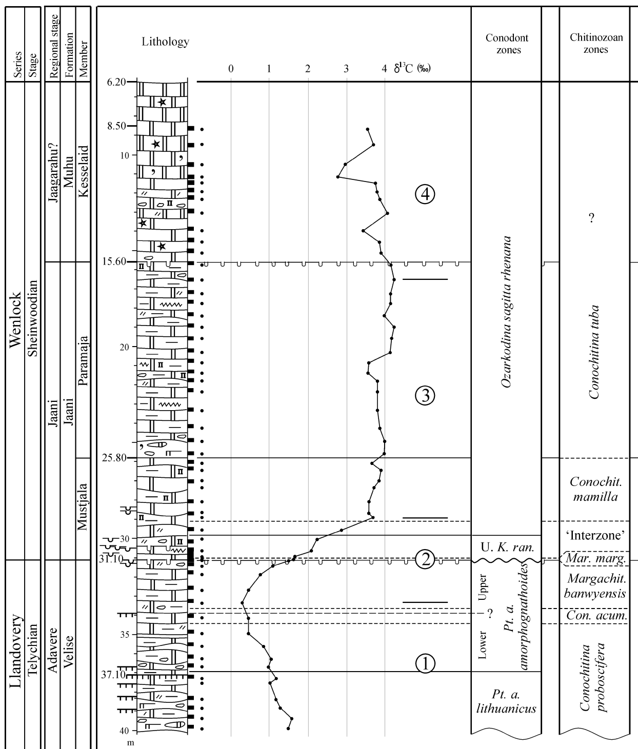
Fig. 6. Carbon isotopes and integrated biostratigraphy in the Suigu (S-3) core section. Dots just right of the micropalaeontological samples indicate the levels of \delta^{13}\text{C} analyses; numbers in circles right of the \delta^{13}\text{C} curve indicate characteristic intervals of the curve discussed in the text. U. K. ran. , Upper Kockelella ranuliformis ; Pt. a. , Pterospathodus amorphognathoides ; Mar. marg. , Margachitina margaritana ; Con. acum. , Conochitina acuminata . For legend see Fig. 2.
