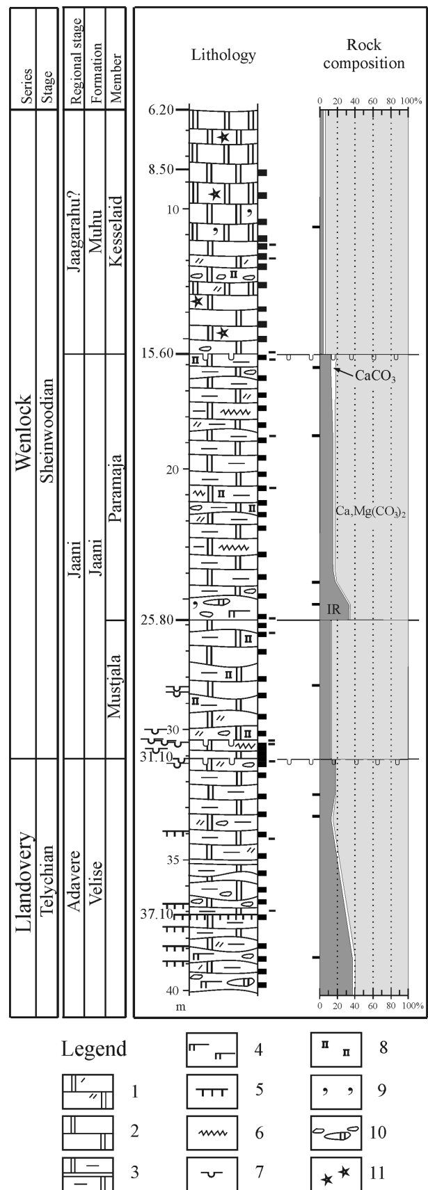
Fig. 2. Suigu (S-3) core section. From left to right: general stratigraphy, regional stratigraphy, lithological log of the section, location of micropalaeontological samples, location of thin sections, rock composition (positions of samples analysed are indicated on the left side). Legend: 1, dolostone (crystal size more than 0.01 mm) with fine and coarse bioclasts; 2, dolostone with crystal size less than 0.01 mm; 3, argillaceous dolostone with interbeds of dolomitic marlstone; 4, dolomitic marlstone; 5, K-bentonite; 6, bioturbation; 7, discontinuity surface; 8, pyritic mottles; 9, glauconite grains; 10, carbonate clasts; 11, vugs. IR, insoluble residue.
