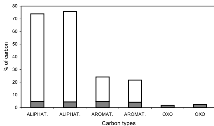
Fig. 3. Distribution of carbon types in the kerogen model (left columns), and in the intact kerogen (right columns). Carbons attached to oxygen are shown shaded. Carbonyl carbon includes carboxylic as well
