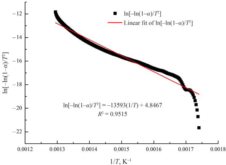
Fig. 2. Linear fitting result of \ln[-\ln(1-\alpha)/T^2] and 1/T .
