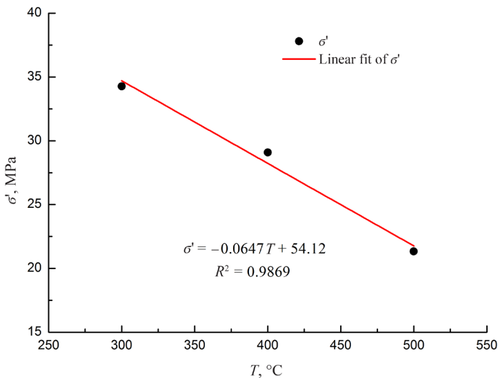
Fig. 3. Linear fitting result of the oil shale skeleton compressive strength and temperature.
