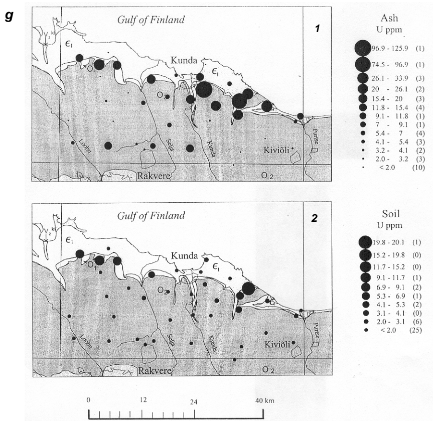
Fig. 2. Distribution of elements in ash (1) and soil (2) for: a – Cd; b – Cu; c – Fe; d – Mo; e – Pb; f – Zn; and g – U. In brackets the number of respective sampling points (designed by V. Mõtus)
