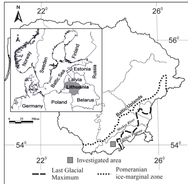
Fig. 1. Location of the study area. Glacial limits according to R. Guobytė (Guobytė and Satkūnas 2011).
